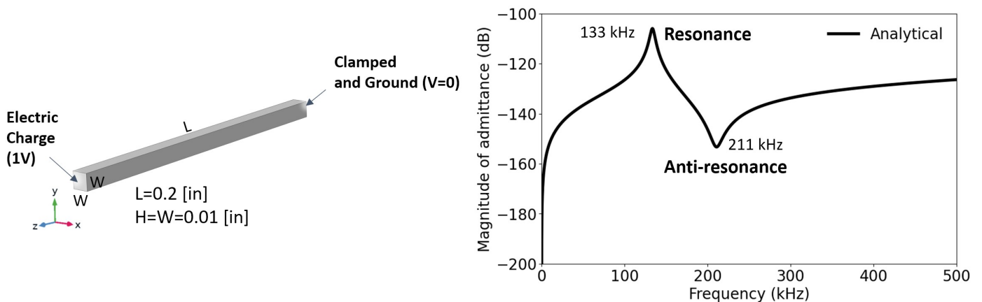
Figure 1 : Admittance Spectrum of PZT Slender Bar
