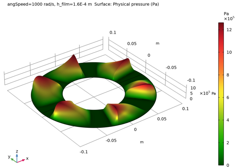
Figure 2: Fluid film pressure profile at \Omega = 1000 rpm with a film thickness of 160 \mu\text{m} .
