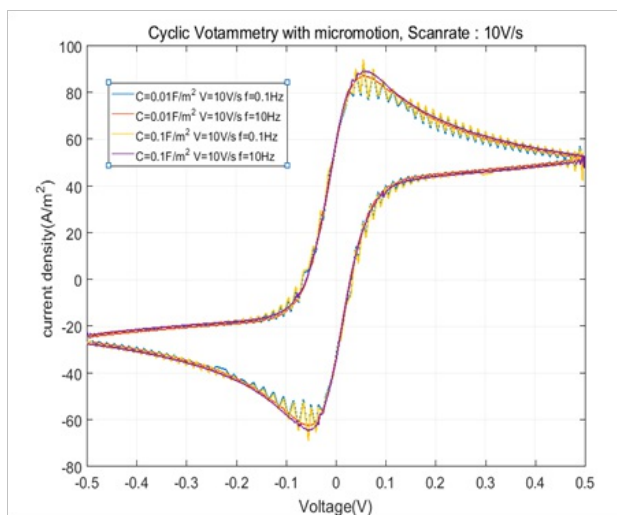
Figure 1: Cyclic voltammometry with mechanical motion
